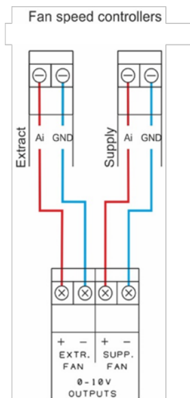
Fig.2.7 Example. Extract & Supply 0-10V output to fan speed controller.
