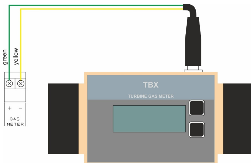
Fig.2.4 Gas meter wiring.
