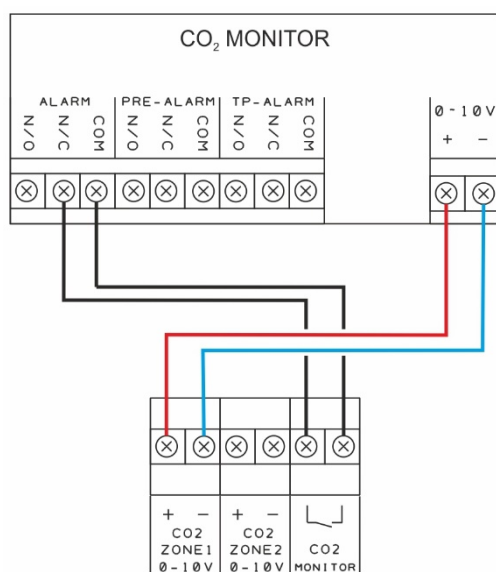
Fig.2.3 CO 2 monitor - wiring to 3000S panel.
