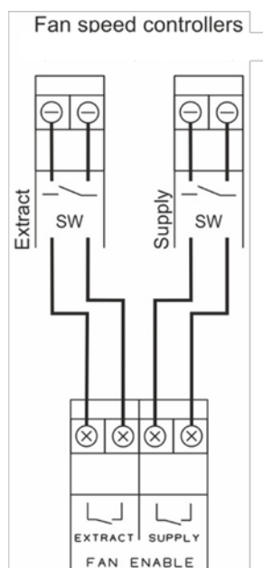
Fig.2.0 Example: Extract & Supply fan speed controller.
