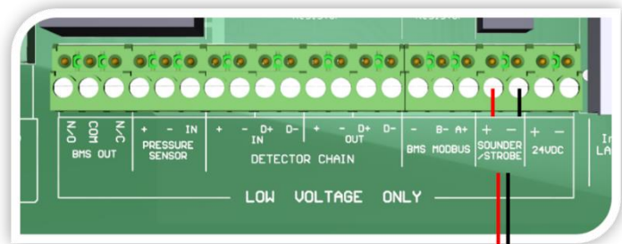
24V DC Output to Sounder/ Strobe Alarm
