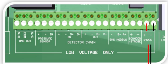
Permanent 24V DC Output
